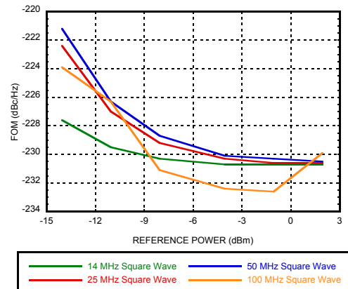
Figure 26. Reference Input Sensitivity, Square Wave, 50 Ω [3]
